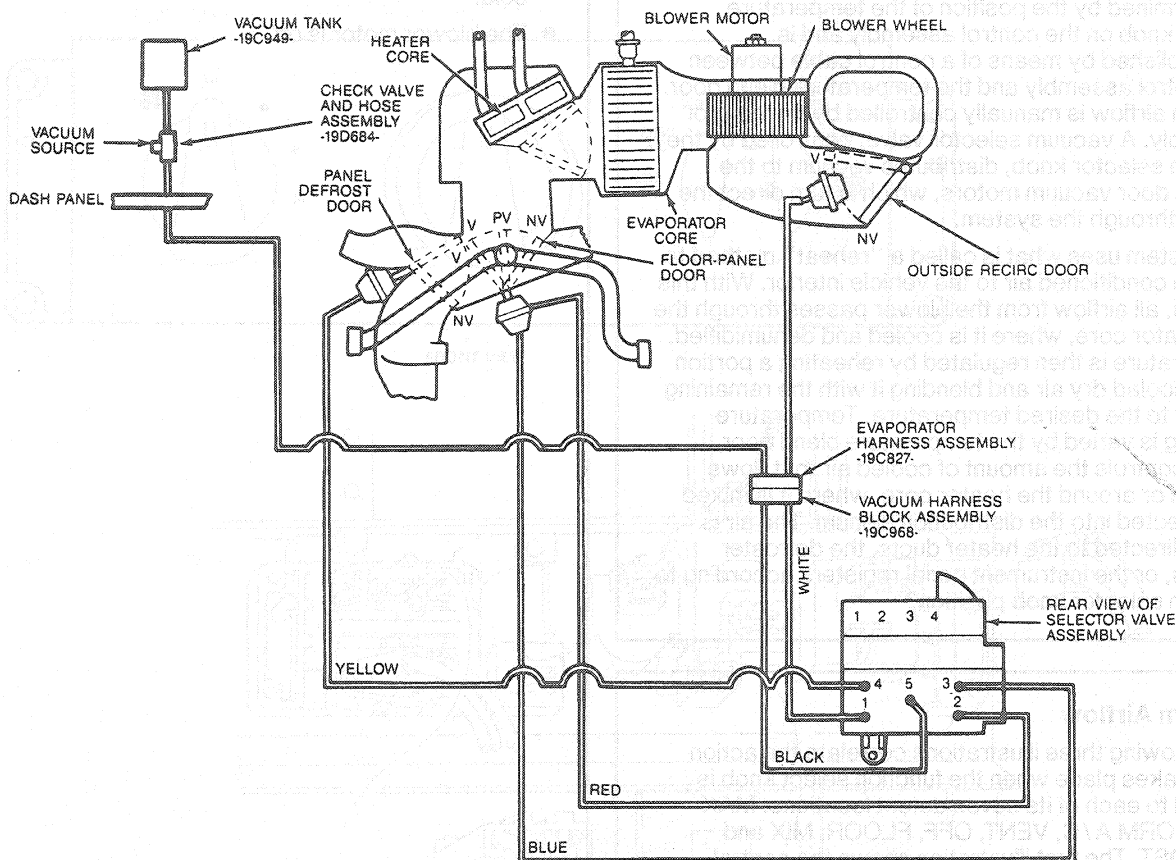
A/C System Schematic and Vacuum Control Chart
