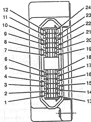
INTEGRAL CONNECTOR
