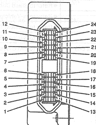
INTEGRAL CONNECTOR
