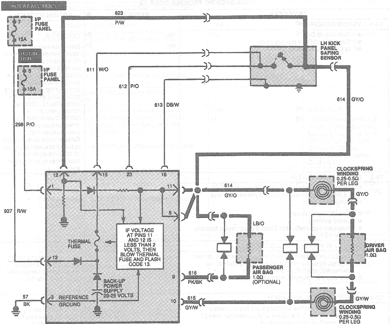
Electrical Schematic—Diagnostic Trouble Code 13
