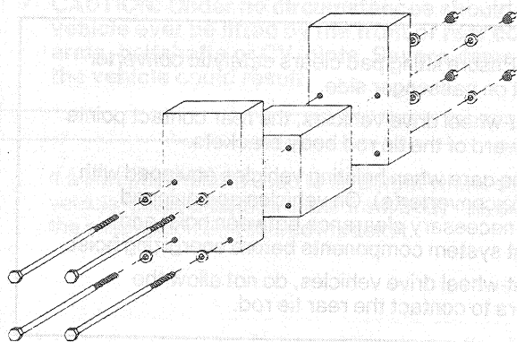
SPACER BLOCKS
