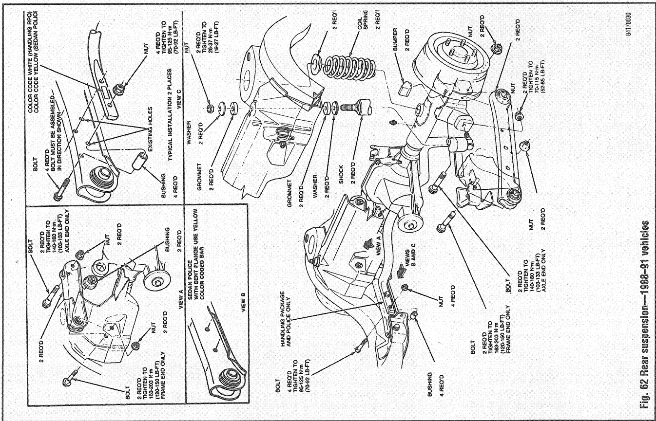
Fig. 63 Rear suspension—1992-93 vehicles, except air suspension
