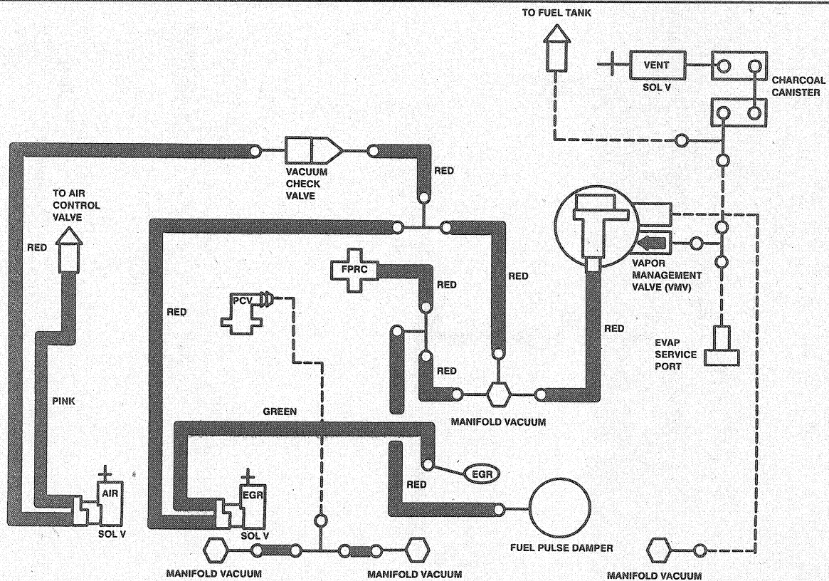
Fig. 120 1998 Mark VIII typical vacuum diagram—4.6L engine
