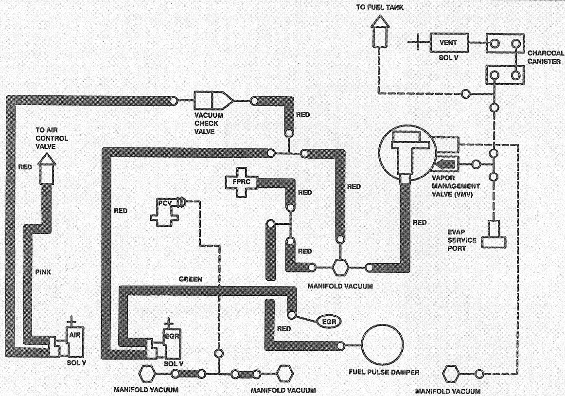
Fig. 119 1997 Mark VIII typical vacuum diagram—4.6L engine
