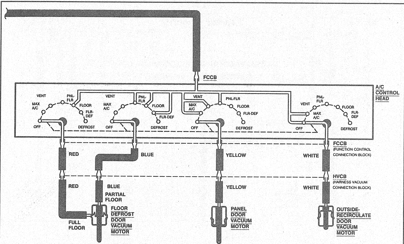
Fig. 109 1995 Mark VIII typical vacuum diagram—4.6L engine (2 of 3)
