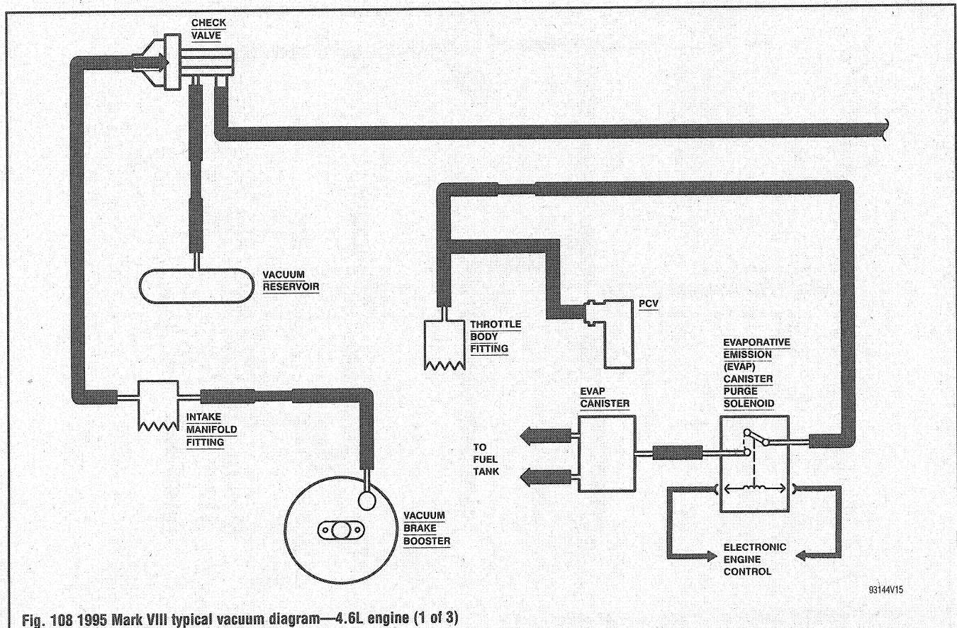
Fig. 107 1995 Continental typical vacuum diagram—4.6L engine
