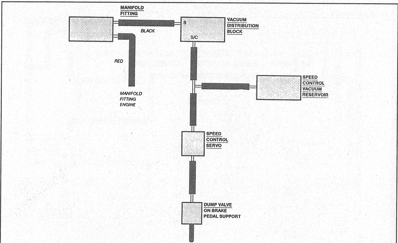
Fig. 101 1994 Continental typical vacuum diagram—3.8L engine
