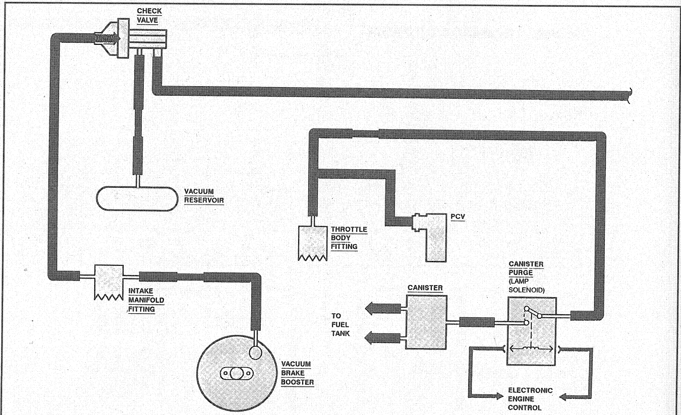
Fig. 102 1994 Mark VIII typical vacuum diagram—4.6L engine (1 of 3)
