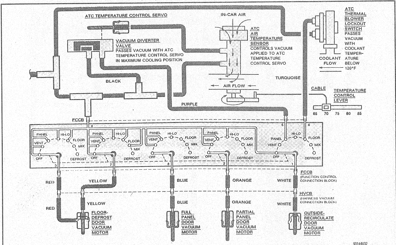
Fig. 86 1988-1990 Town Car typical vacuum diagram—5.0L engine (2 of 2)
