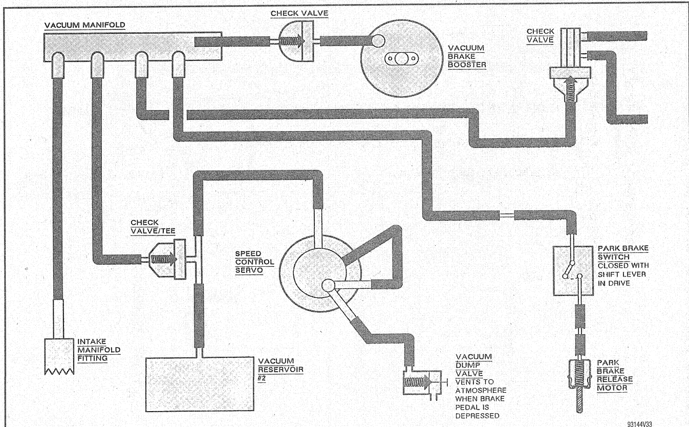
Fig. 87 1991 Town Car typical vacuum diagram—4.6L engine (1 of 2)
