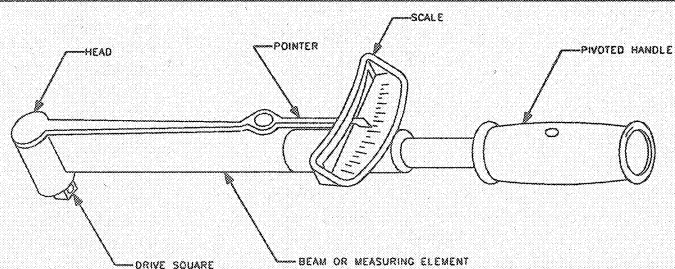
Fig. 27 Example of a beam type torque wrench
